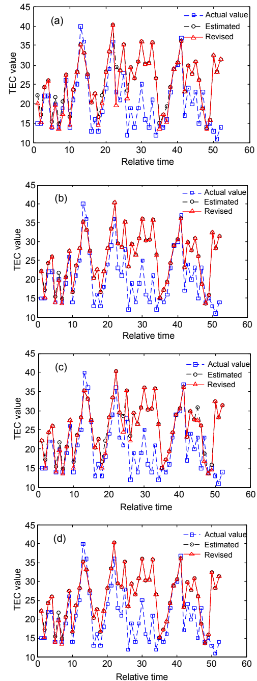
Fig. 14 Updating results with conditions TF (a), TS (b), FS (c), and TFS (d) in structure 1
